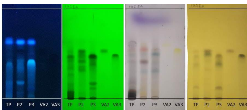
Hệ dung môi 100% ethyl acetat
